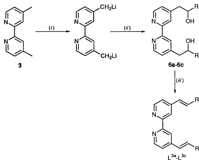
Scheme 3 R as in Scheme 2. (i) 2\text{LiNPr}^t_2 ; (ii) 2\text{RCHO} ; (iii) ptps
