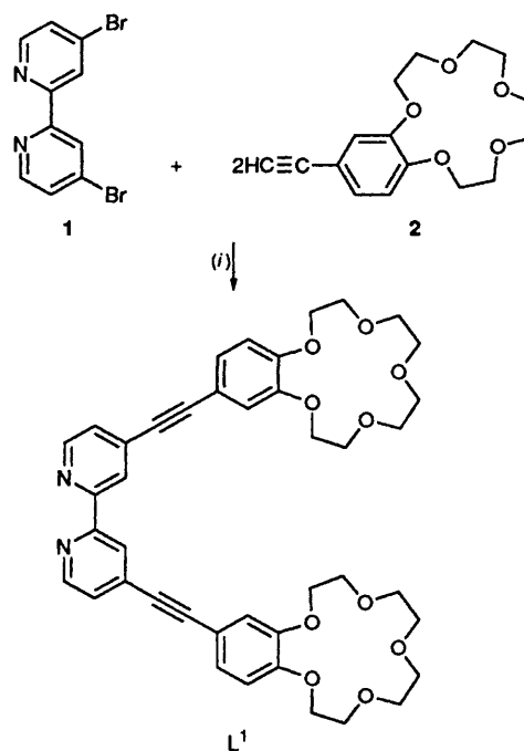
Scheme 1 (i) [\text{Pd}(\text{PPh}_3)_2\text{Cl}_2] , CuI, NEt 3
