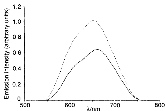
Fig. 4 Fluorescence-emission spectrum (—) of a film of poly-[RuL 2a ] 3 ] 2+ coated onto an optically transparent conducting glass electrode in acetonitrile at 298 K. The broken line shows the emission spectrum after addition of an excess of Mg 2+ [as Mg(ClO 4 ) 2 -acetonitrile solution]. Excitation wavelength = 450 nm
